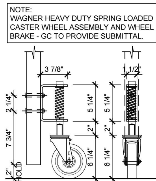
08 CASTER WHEEL SCALE: 1 1/2\"/>
