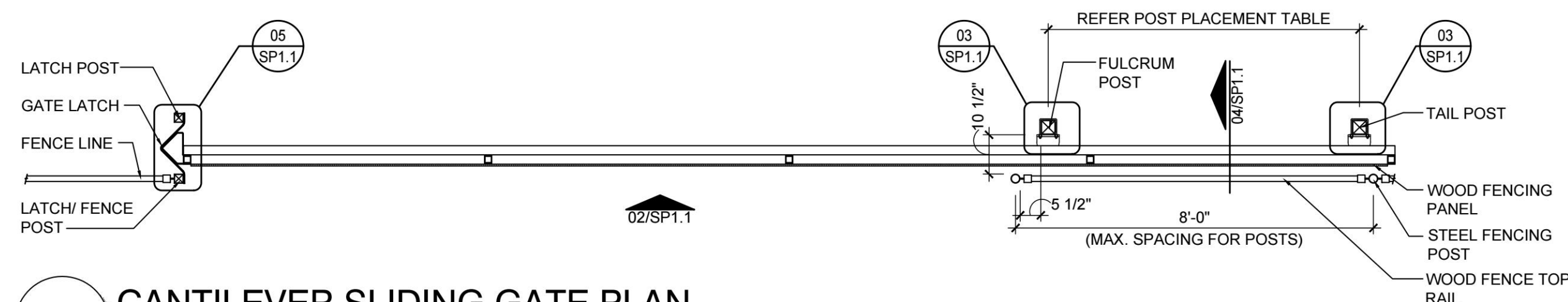
01 CANTILEVER SLIDING GATE PLAN SCALE: 3/8\"/>
