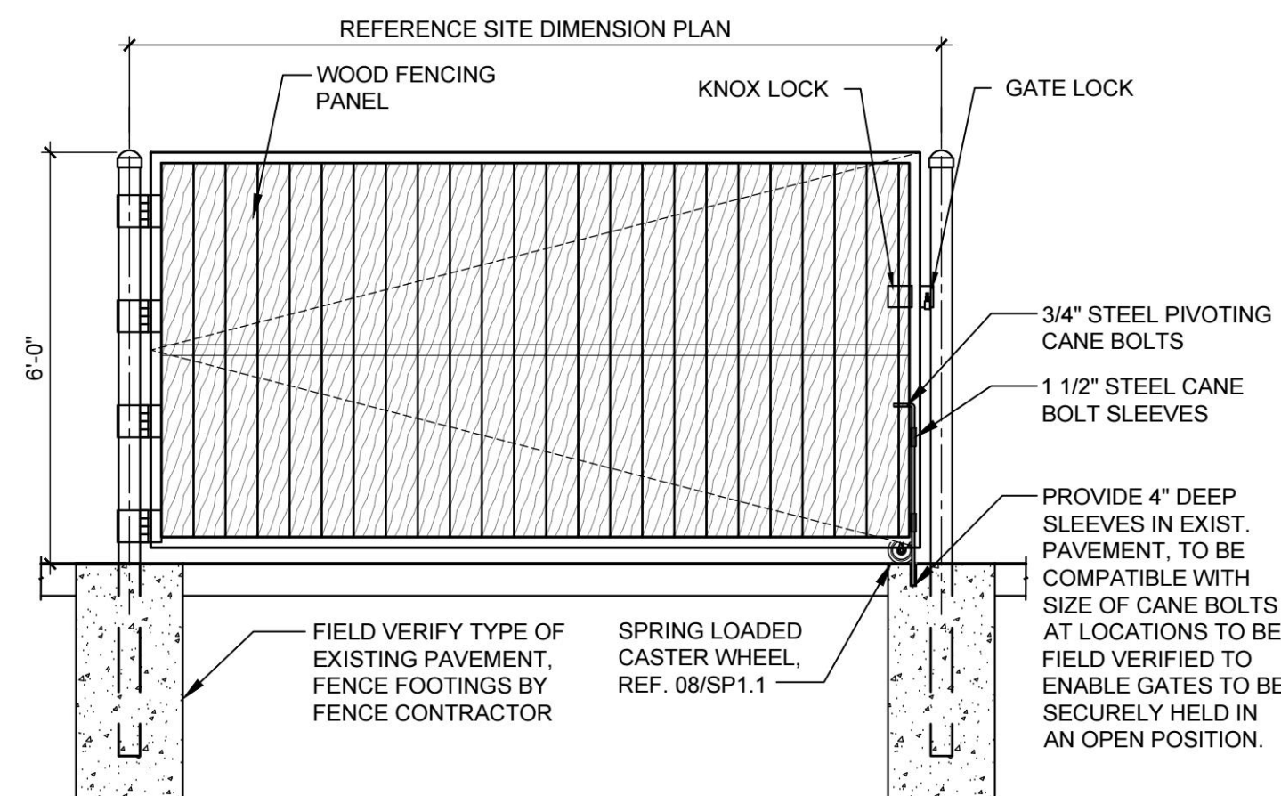
06 SWING FENCE GATE ELEVATION SCALE: 3/8\"/>
