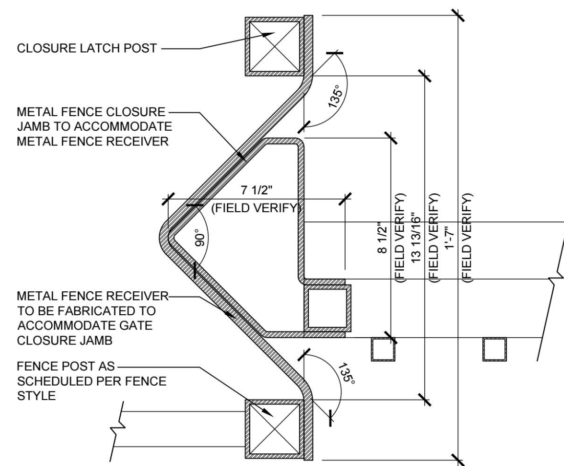
05 FENCE RECEIVER DETAIL SCALE: 3\"/>
