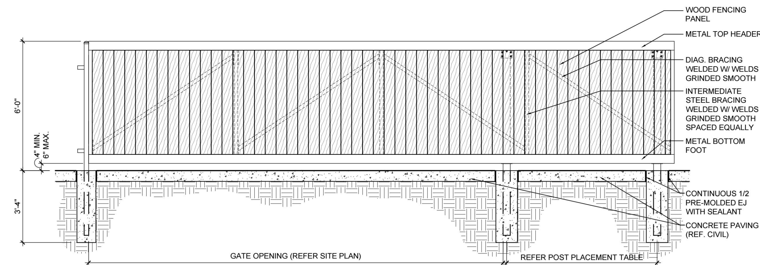
02 CANTILEVER SLIDING GATE ELEVATION SCALE: 3/8\"/>
