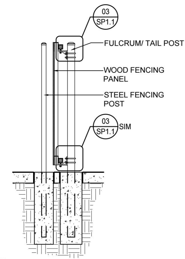
04 GATE SECTION SCALE: 3/8\"/>
